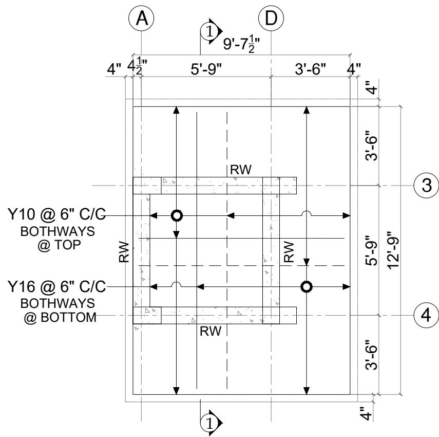
PLAN OF FOOTING - "CF6" LIFT PIT (9'-0" x 10'-6" x 1'-6")
